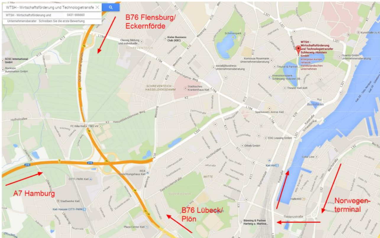
google maps
